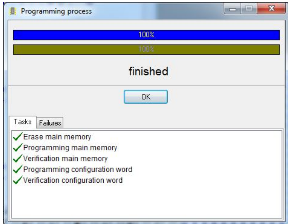
Figure 9. Programming process screen of ASIX UP - successful programming
