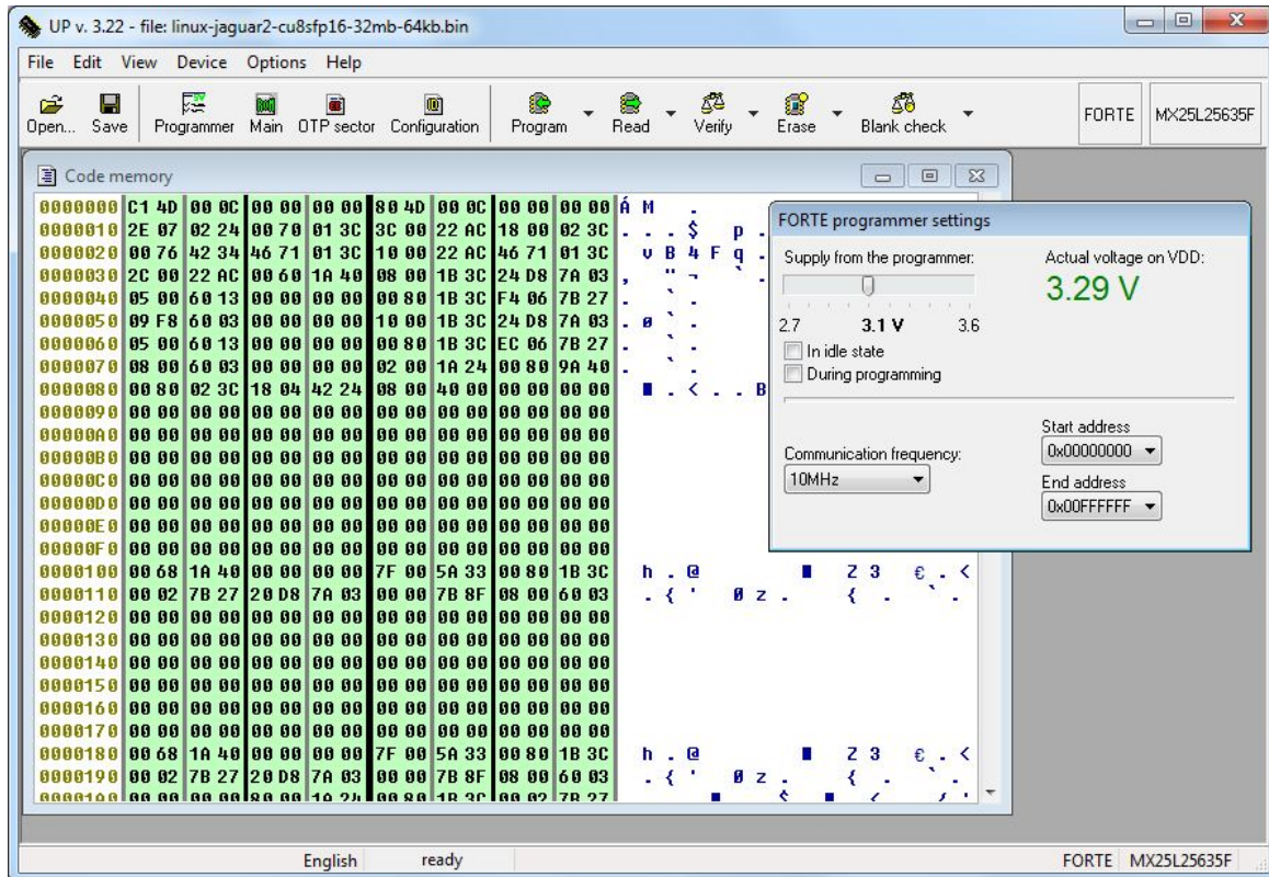
Figure 6. Main screen of ASIX UP
